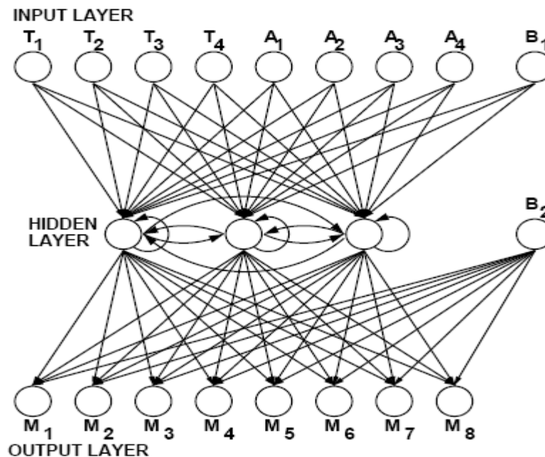
Fig. 3.3 The neural network architecture used for the quadrupedal robot.
