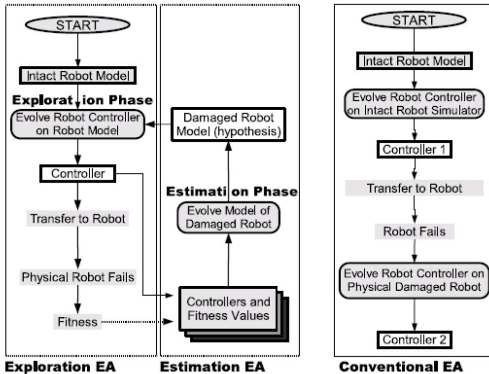
Fig. 3.1 Flow chart of estimation-exploration phases
