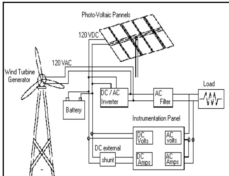
Fig. 2. A simple Hybrid Solar & Wind System
