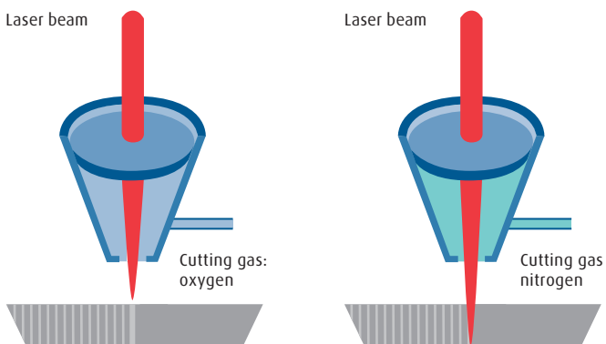
Fig. 11: Focus position for oxygen-cutting compared to high-pressure nitrogen-cutting
