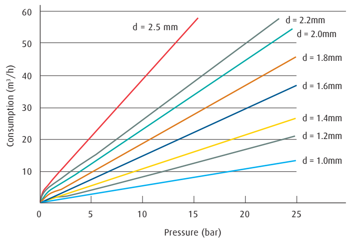
Fig.12: Consumption of nitrogen depends on the gas pressure in the nozzle and the size of the nozzle, d
