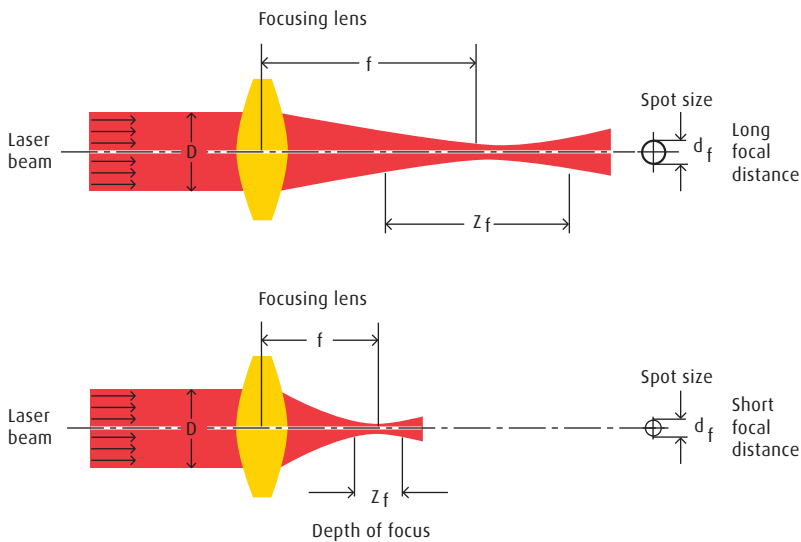
Fig. 3: Focusing a laser beam
