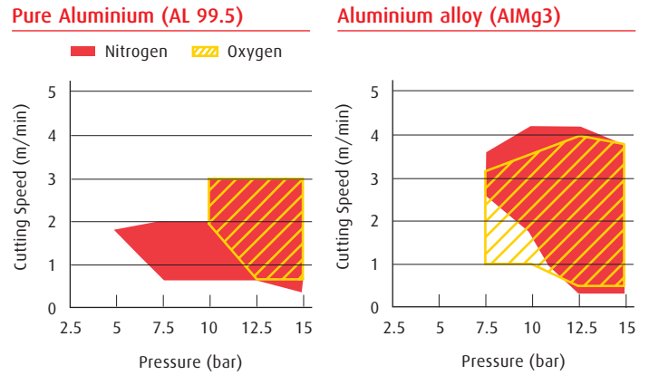
Fig. 13: Dross-free parameter ranges when using nitrogen and oxygen up to 15bar for cutting 2mm pure aluminium and 2mm aluminium alloy, laser power 1500W
