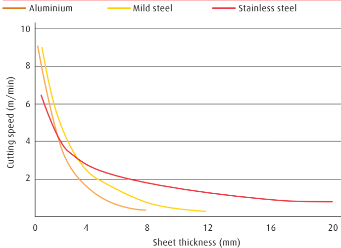
Fig. 2: Typical cutting rates with approximately 3kW of laser power
