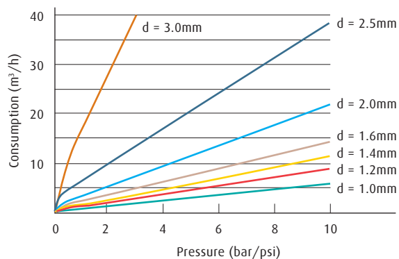
Fig. 10: Consumption of oxygen depending on the gas pressure in the nozzle and the size of the nozzle, d
