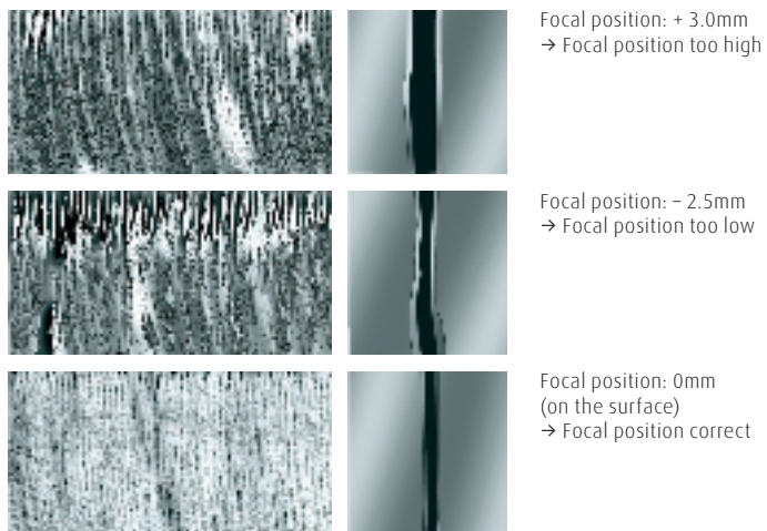
Fig. 6: Effect of focal position on cutting performance
