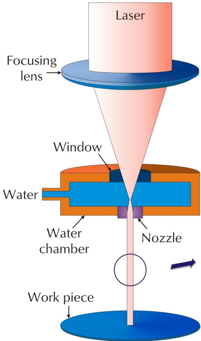
Laser guided by total internal reflection
